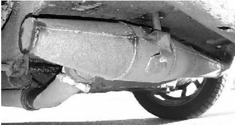
XP-exhaust system with the long reverse cone
