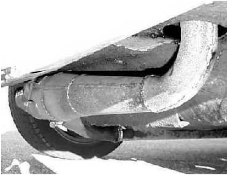
Tuned XP-exhaust system ready to go
